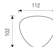
Pouf top view
